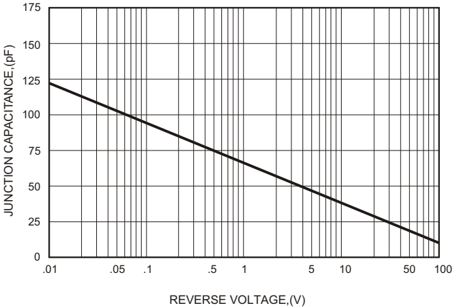
FIG.6-TYPICAL JUNCTION CAPACITANCE
